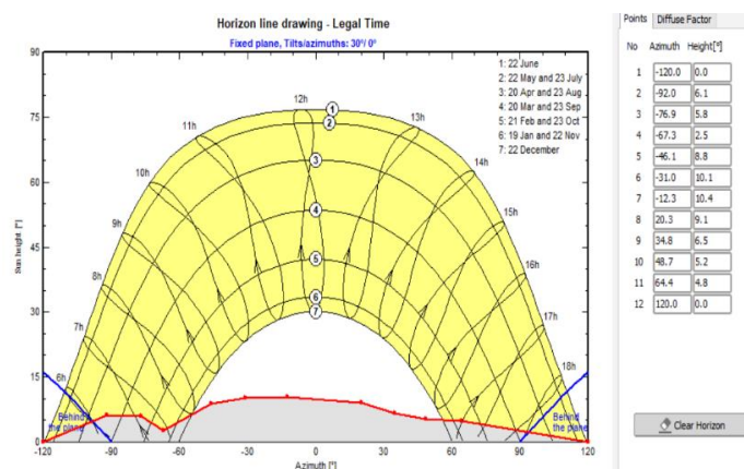
Fig. 1. Horizon profile at the Abbasabad site.
