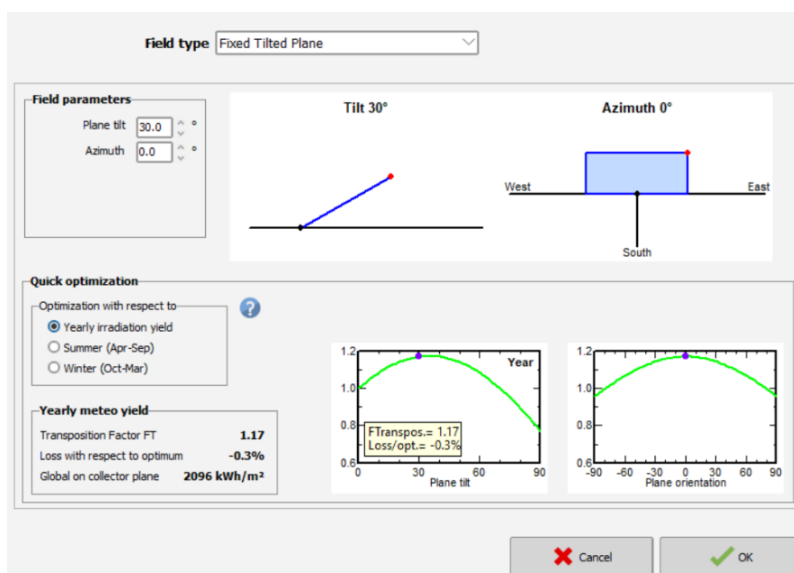
Fig. 2. Determination of panel tilt angle in PVsystem.
